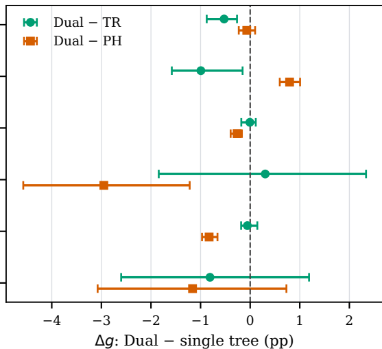
(b) Dual versus independently trained single tree
